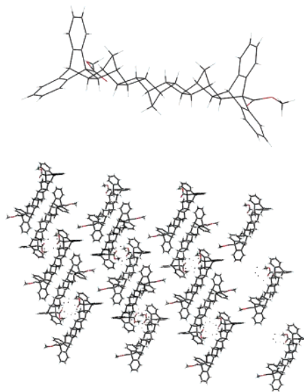
Figure 2. X-ray crystal structure of the syn trimer diester in Scheme 1.
