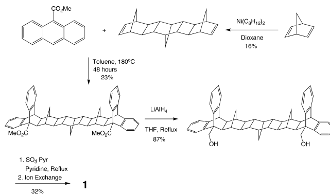
Figure 1. Synthesis of 1 .
